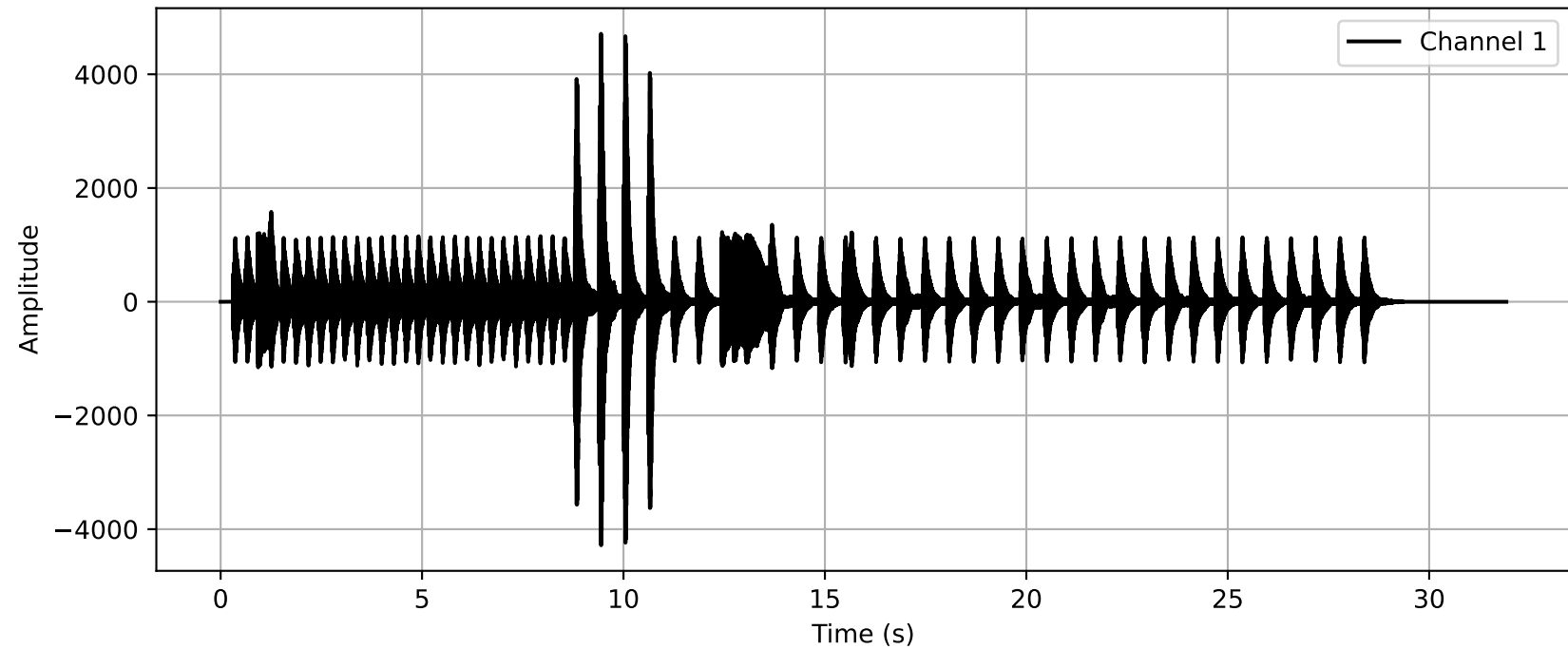
Waveform of Baricitinib.wav
